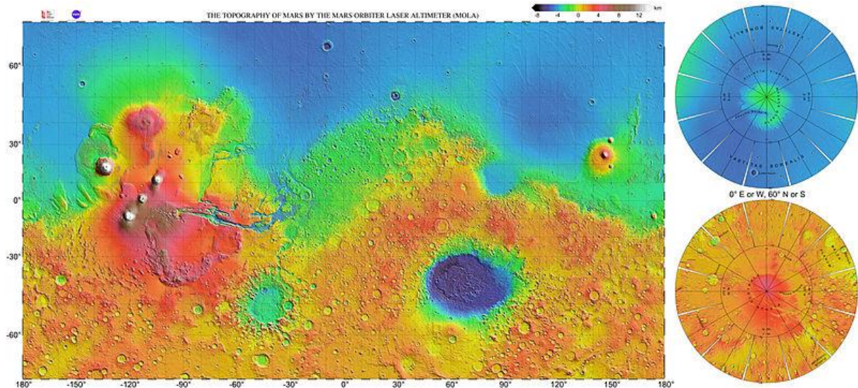
Fig. 2. Very high resolution topographic shaded relief map of Mars (Vestitas Borealis Basin), made by the Mars Orbiter Laser Altimeter (MOLA) data taken from the Mars Global Surveyor spacecraft. The map has a resolution 0.125° (300 dots per inch) and is shown as a Mercator projection to latitude 70° north and south. The original NASA image has been modified by increasing the font size of the map grid and elevation key labels. Polar regions are added from enlarged crops of PIA02993; the areas from 60° to 75° latitude are in the transverse Mercator projection, and those from 75° to 90° latitude are in the Lambert azimuthal equal-area projection. Some of the features in this image have been annotated in Wikimedia Commons. Likewise, operational landrovers traipsing the Martian surface, NASA's Opportunity and Curiosity vehicles, have delivered invaluable visual documentation of the red planet's territorial features.
